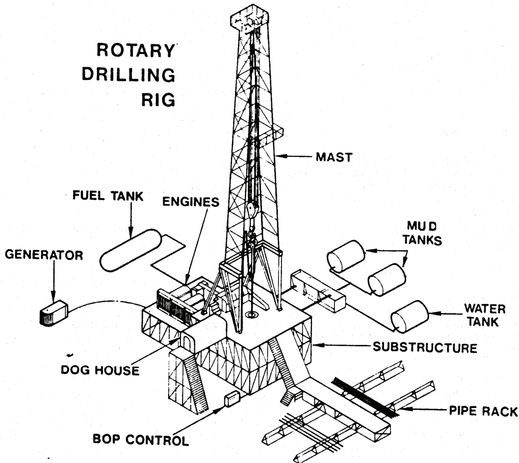
FIGURE D-1: TYPICAL DRILL SITE MATERIALS AND EQUIPMENT.
